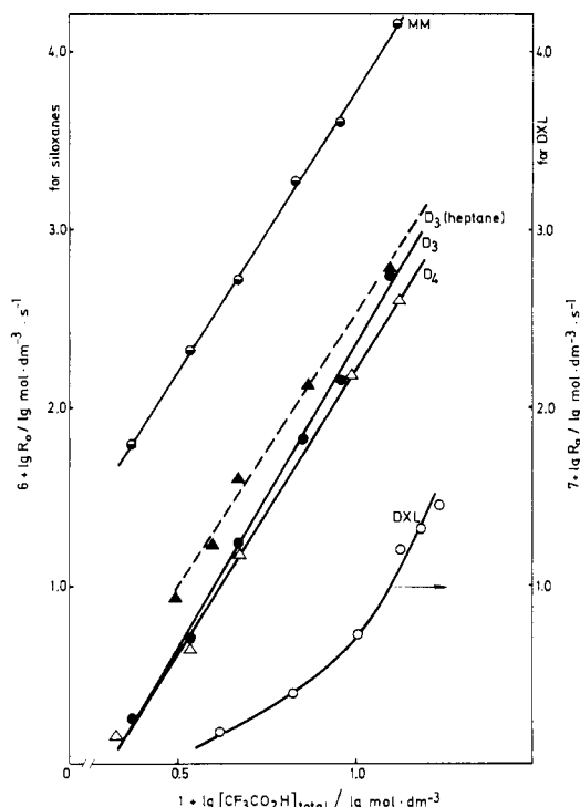
Figure 1. Dependence of the initial rate of acidolysis of siloxane and acetal monomers with trifluoroacetic acid in methylene chloride (continuous line) and in heptane (dashed line) at 35 °C on the total initial concentration of the acid. Initial concentration of the monomer is a constant 2.0 \text{ mol dm}^{-3} . Experimental points: (○) DXL; (●) MM; (Δ) D 4 ; (●) D 3 (all in \text{CH}_2\text{Cl}_2 ); (▲) D 3 (in heptane). The ordinate scale for DXL is marked at the right side.
